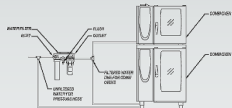
TYPICAL WATER CONNECTION DETAIL FOR COMBI OVEN NTS
